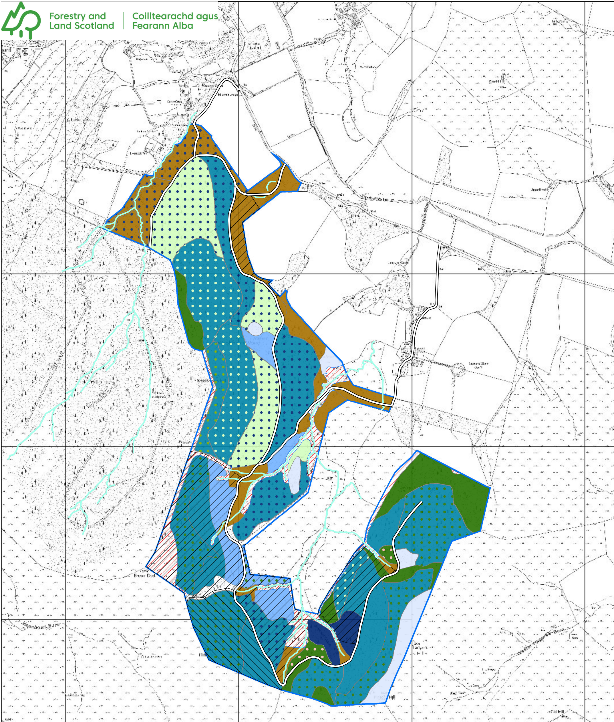
Map 6: Future Habitats and Species
